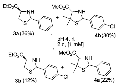
Scheme 3. Metathesis of Thiazolidines a
