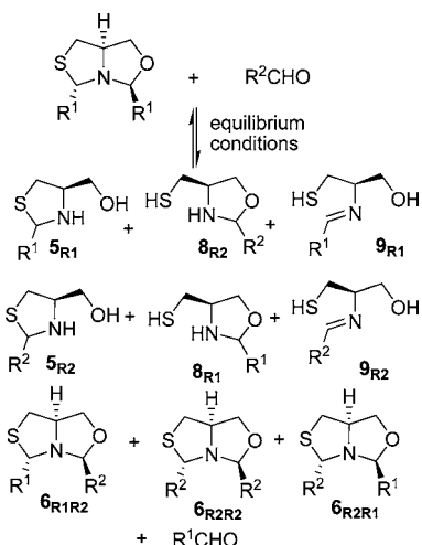
Scheme 5. Potential Library of Thiazolidine–Oxazolidine Heterocycles
