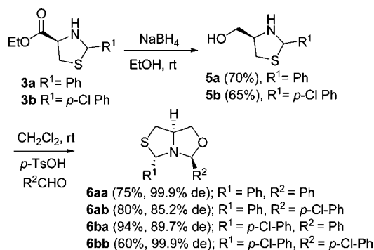
Scheme 4. Synthesis of Fused Thiazolidine–Oxazolidine Heterocycles
