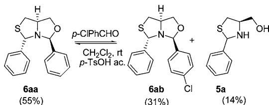
Scheme 6. Exchange Reaction of Bicycle 6aa a
