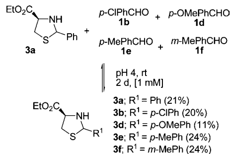
Scheme 2. Exchange Reaction between Thiazolidines 3a and Aldehydes 1b,1d–f a
